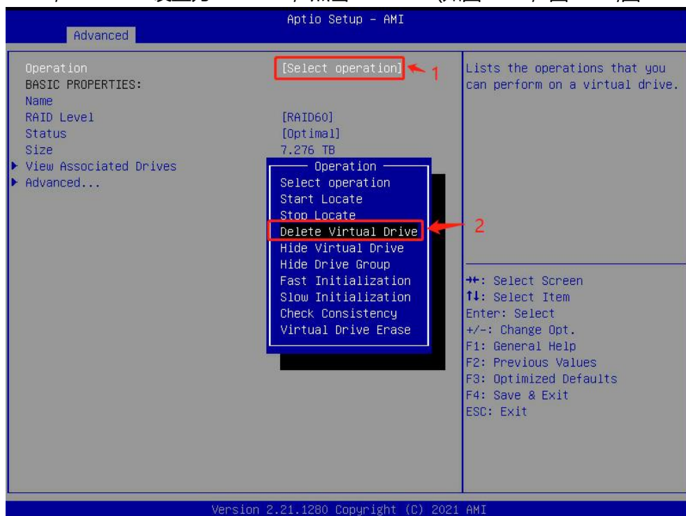
图 7-44 选择 “Delete Virtual Drive”
